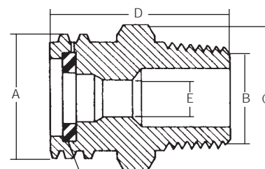
Gasket (Furnished with adapter)
