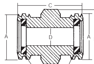
Gasket (Furnished with adapter)
