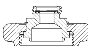
5776 Reducer Coupling
